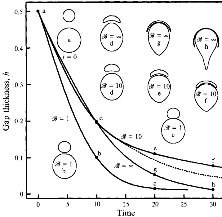
FIGURE 6. The rate of film drainage versus time for drops with Bond numbers \mathcal{B} = 1, 10 and \infty ; \lambda = 1 ; a_1/a_2 = 2 . The solid curve corresponds to the thickness of the film on the axis of symmetry, r = 0 , and the dashed curve corresponds to the minimum film thickness. Drop shapes at different times are shown for reference.
