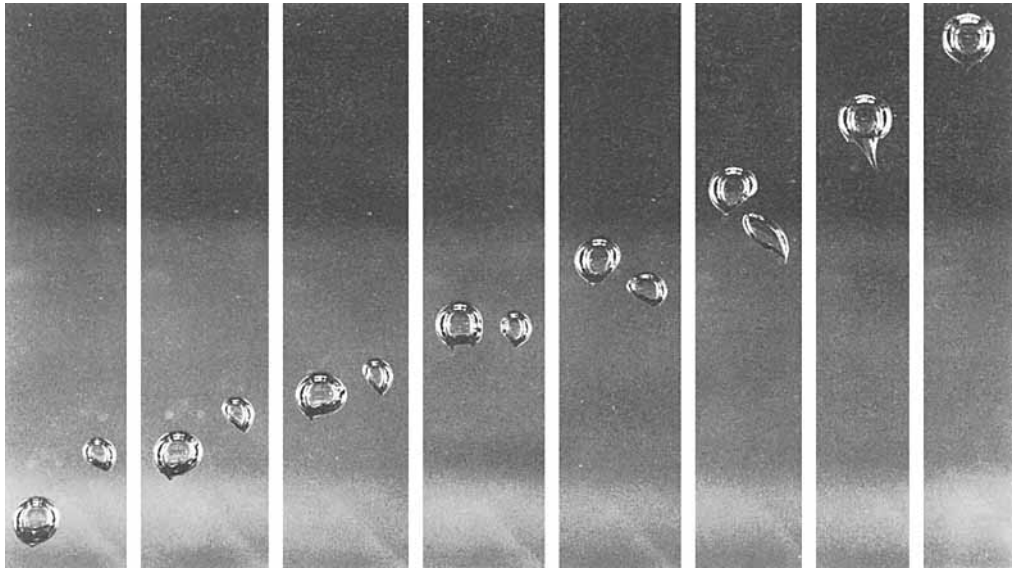
FIGURE 12. Sequence of photographs showing the interaction of initially offset air bubbles in corn syrup, with \mathcal{B} \approx 50 and \mathcal{R} \approx 5 \times 10^{-3} . Photographs are shown at 10 s intervals. The bubbles coalesce within about 30 s after the last photograph shown.
