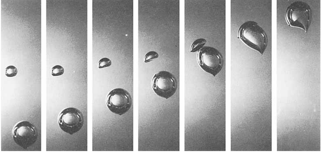
FIGURE 11. Sequence of photographs showing the interaction of initially offset air bubbles in corn syrup, with \mathcal{B} \approx 50 and \mathcal{R} \approx 5 \times 10^{-3} . Photographs are shown at 5 s intervals. The bubbles coalesce about 10 s after the last photograph shown.
