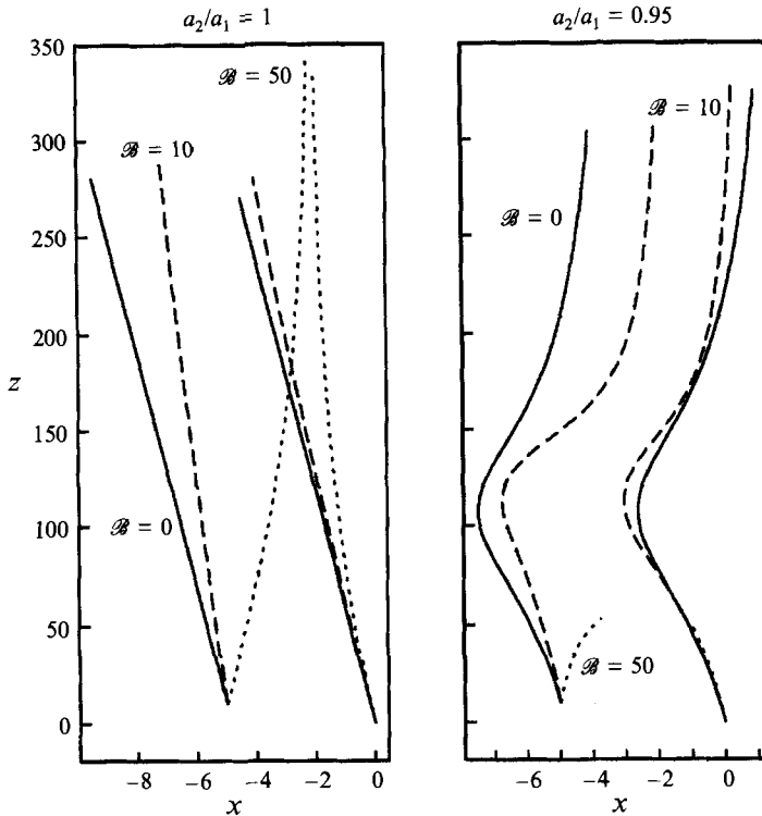
FIGURE 21. Trajectories of two bubbles ( \lambda = 0 ) for different values of the Bond number and bubble sizes, in the limit of small deformation. The solid lines are for \mathcal{B} = 0 , the dashed lines for \mathcal{B} = 10 , and the dotted lines for \mathcal{B} = 50 . The curves for a_2/a_1 = 0.95 and \mathcal{B} = 10 are stopped when the bubbles have aspect ratios greater than 3/2 . The bubbles are initially separated by a horizontal distance of 5a_1 and a vertical distance of 10a_1 .
