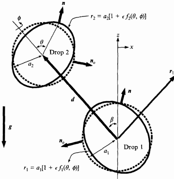
FIGURE 19. Geometry of the two-drop problem and definition of the normals \mathbf{n} and \mathbf{n}_o . Drops 1 and 2 have radii a_1 and a_2 , respectively, are separated by a distance d , and are oriented at angle \beta with respect to gravity.
