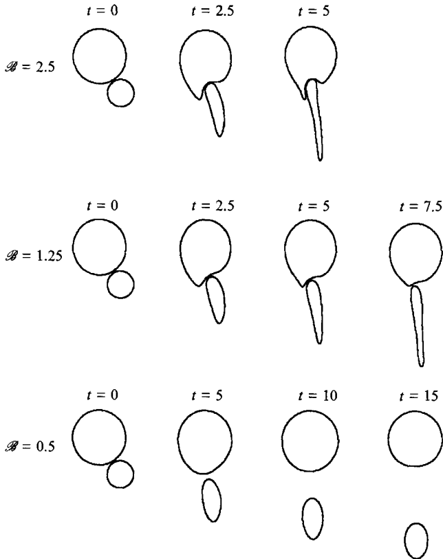
FIGURE 18. The effect of interfacial tension on the interactions between a small drop trailing a larger drop illustrated in a frame of reference moving with the drops. Calculations are shown for \mathcal{B} = 2.5, 1.25 and 0.5 ; \lambda = 0.1 ; a_1/a_2 = 1/2 (Bond number based on the trailing drop). For large enough Bond numbers, the small drop may be sucked into the larger drop owing to the deformation of the larger drop. The horizontal planar surface is not shown.
